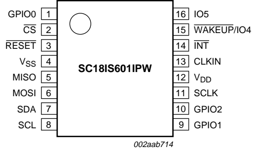
Fig 4. SC18IS601 pin configuration for TSSOP16
