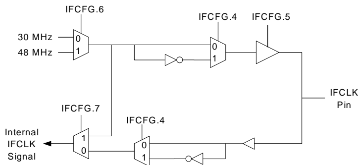
Figure 15-1. IFCLK Configuration
