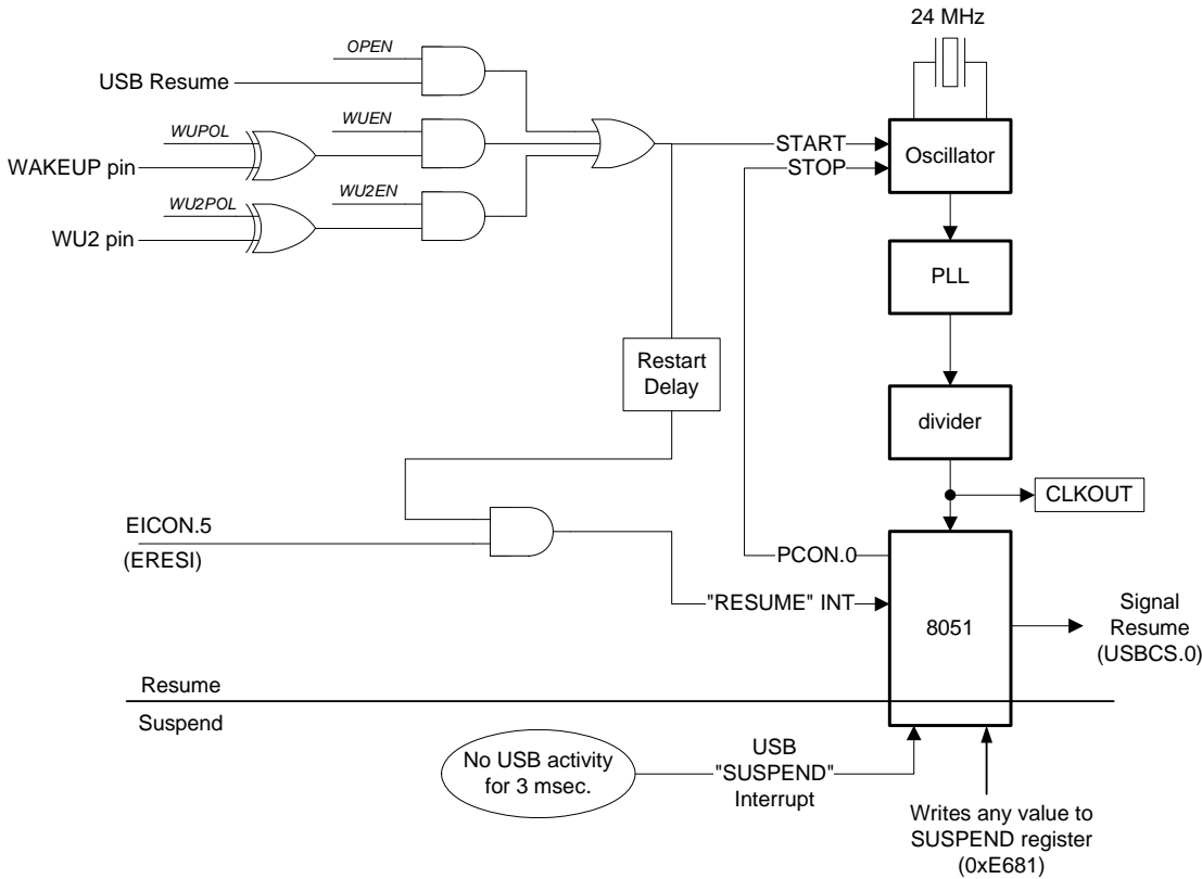
Figure 6-1. Suspend-Resume Control
