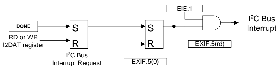
Figure 4-6. I 2 C Bus Interrupt Enable Bits and Registers
