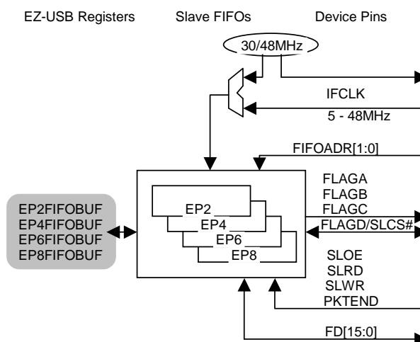
Figure 9-25. EPxFIFOBUF Registers
